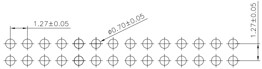
△ Recommended PCB Layout PCB Board Tolerance±0.05
