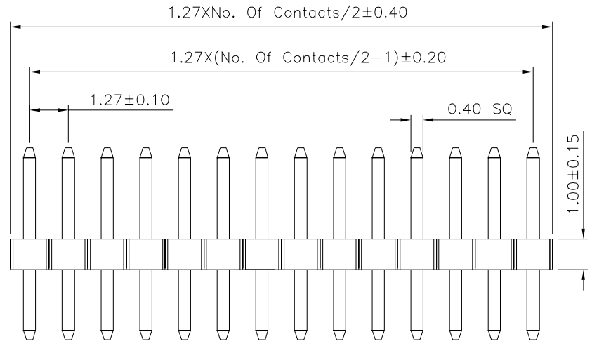
△ 100Pin Warpage:0.25mm Max.
