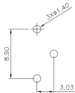
PCB Layout Diagram Top View
