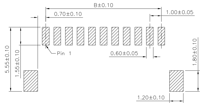
Recommended P.C.B Layout(Top Side) P.C.B Thickness=1.20~1.60mm(Tolerance=±0.05)
