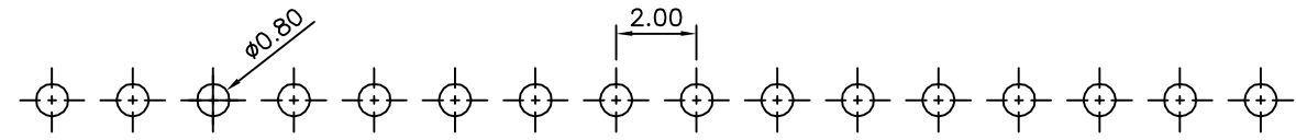
Recommended P.C.B. Layout
