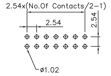
Recommended P.C.Board layout Bottom View
