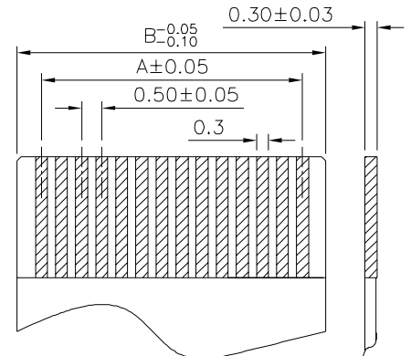
Accommodated FFC/FPC
