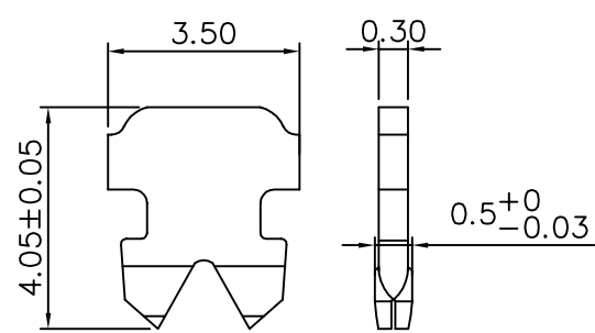
2 Prongs For Solid Wire
