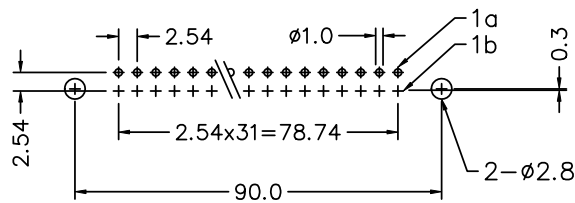
LAYOUT PATTERN
