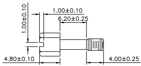
#4-40UNC Hexscrew
