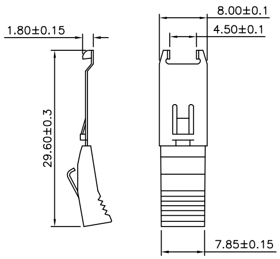
Flag Hooks
