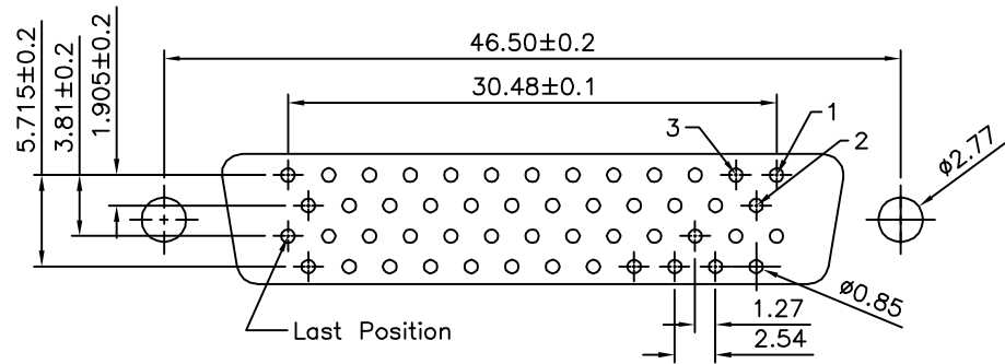
\Delta Recommended P.C.B. Layout
