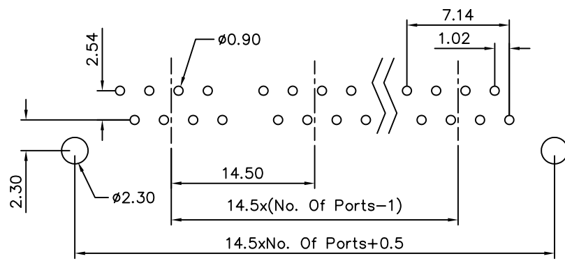
PC Board Layout Ref.
