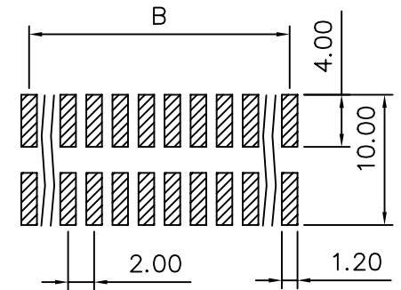
Recommend PCB Layout Top View
