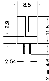
Detail P
