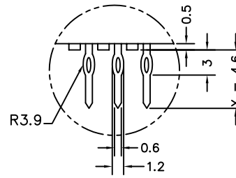
Detail P
