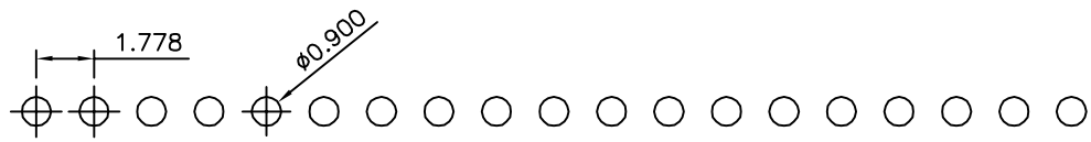
Recommended P.C.B. Layout
