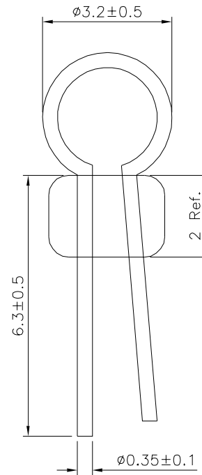
△With Insulator
