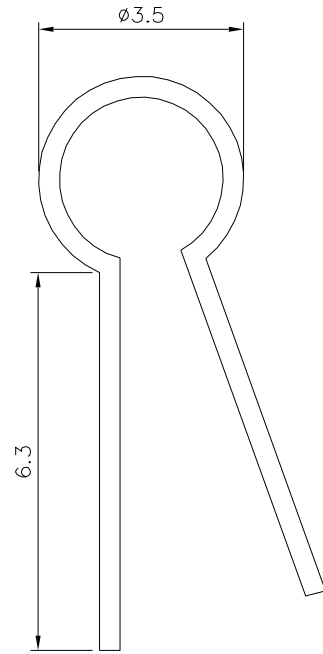
Without Insulator
