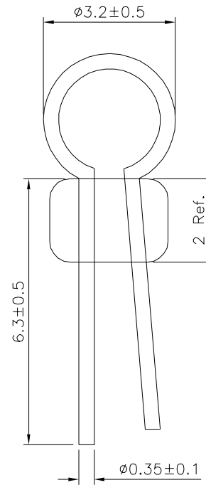
△With Insulator
