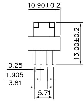
PCB Mounting Dimensions
