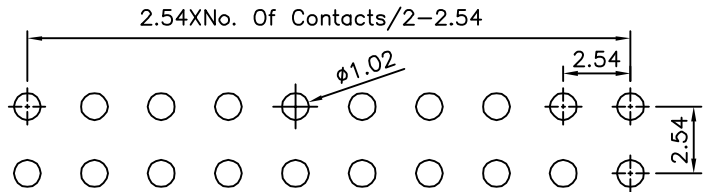
Recommended P.C.B. Layout (Top View) (PCB Board Tolerance ±0.05)
