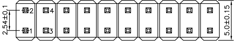
Recommended P.C.B. Layout (Top View) (PCB Board Tolerance ±0.05)
