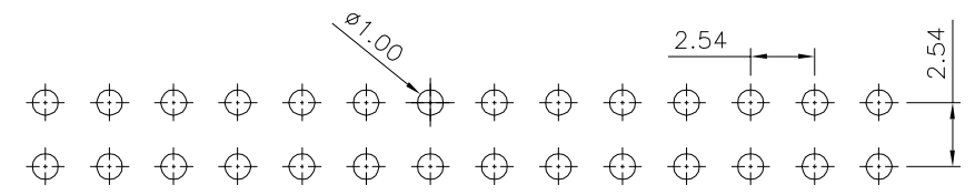
Recommended P.C.B. Layout ⚠️ Tolerance \pm 0.05
