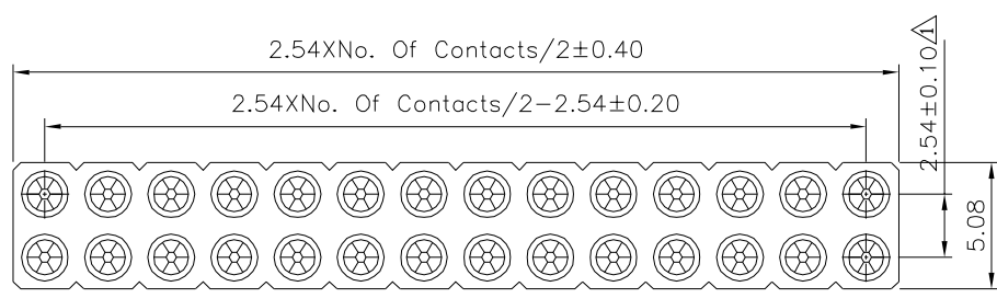
Recommended P.C.B. Layout ⚠️ Tolerance \pm 0.05
