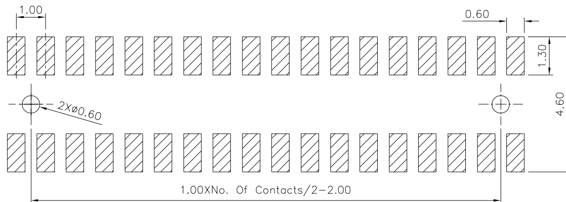
Recommended P.C.B. Layout(Top Side) (PCB Board Tolerance±0.05)
