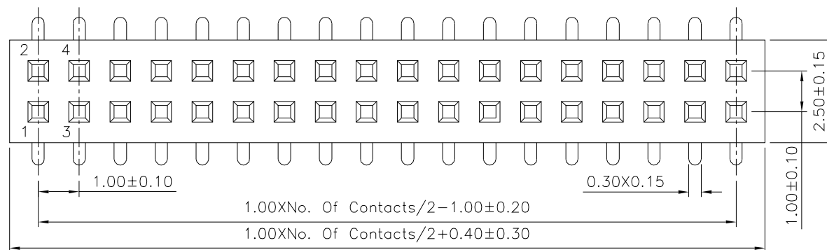
Recommended P.C.B. Layout(Top Side) (PCB Board Tolerance±0.05)
