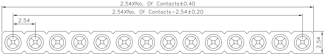
Recommended P.C.B. Layout
