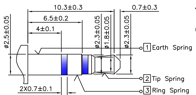
△ Matching Plug
