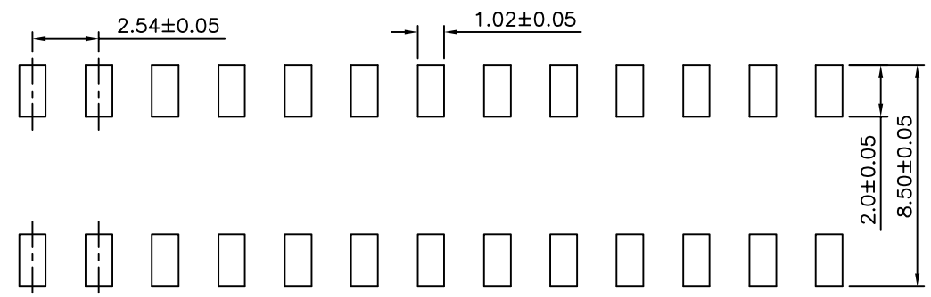
Recommended P.C.B. Layout (PCB Board Tolerance±0.05)
