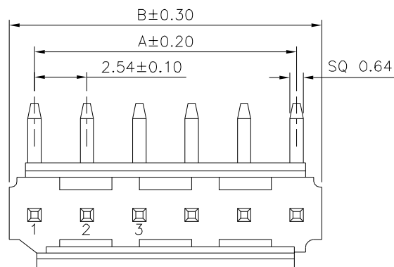
02~06 Pin
