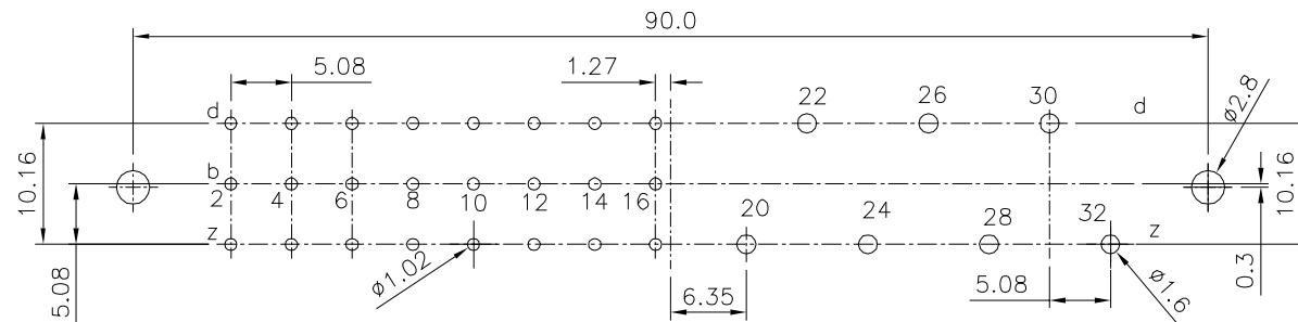
Recommended P.C.B. Layout (PCB Board Tolerance±0.05)
