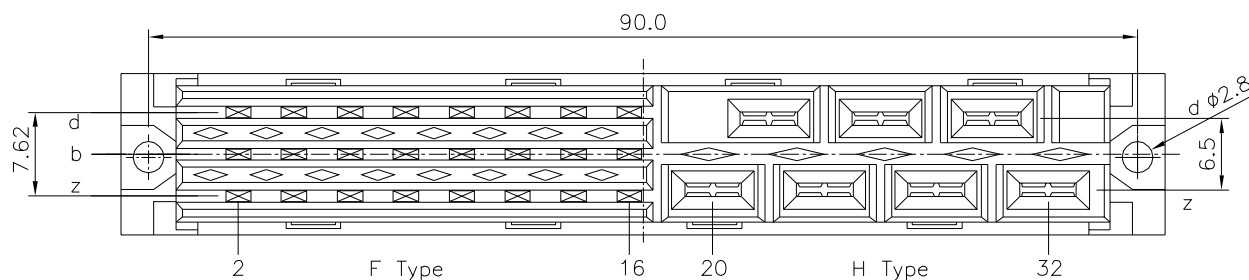
Recommended P.C.B. Layout (PCB Board Tolerance±0.05)
