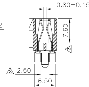
Section K-K
