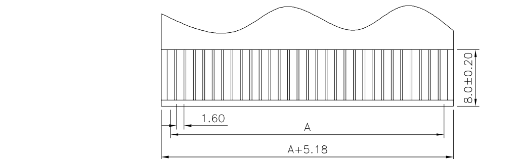
Connecting Finger Layout
