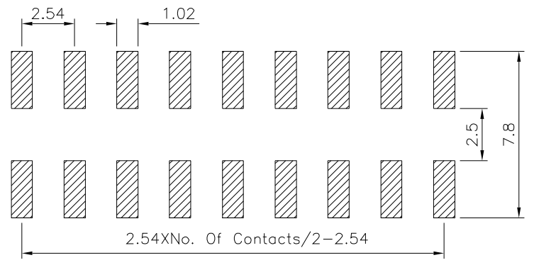
Recommended P.C.B. Layout(Top View) (PCB Board Tolerance±0.05)
