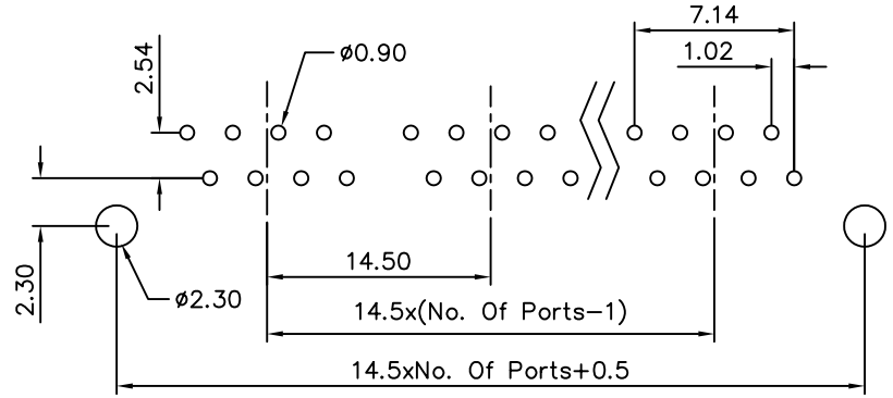
PC Board Layout Ref.
