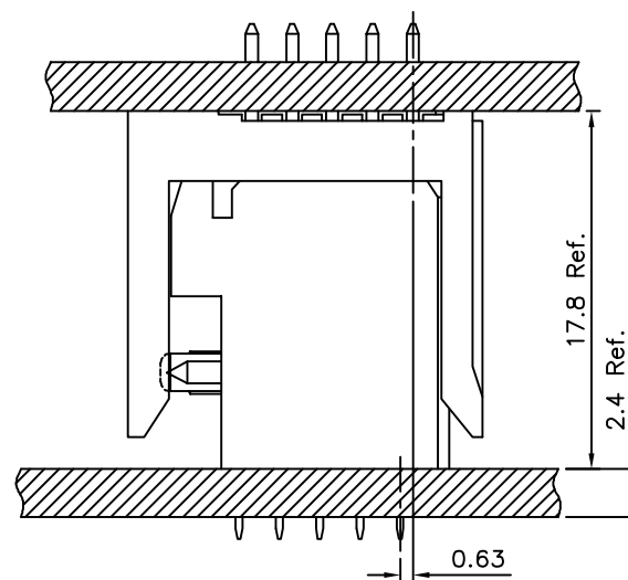
△ Board To Board Offset Application Example
