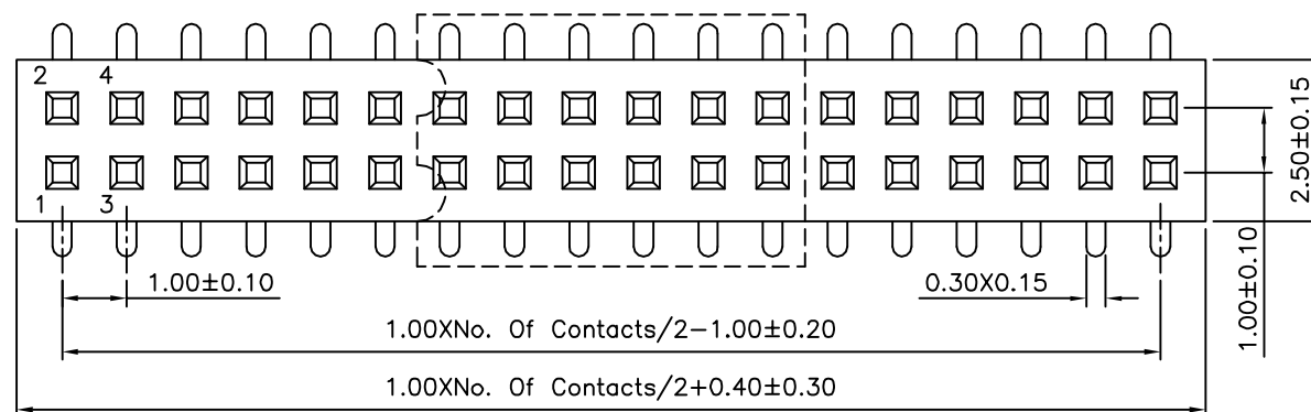
Recommended P.C.B. Layout(Top Side) (PCB Board Tolerance±0.05)
