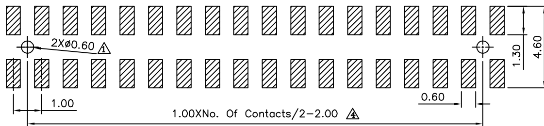
Recommended P.C.B. Layout(Top Side) (PCB Board Tolerance±0.05)
