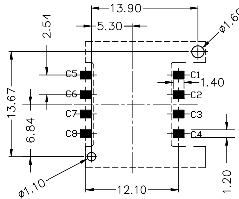
P.C.B. LAYOUT(Tolerance:±0.05mm)
