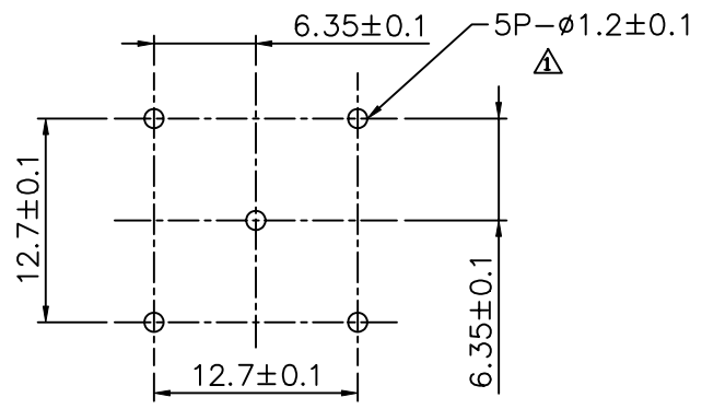
Recommended PC Board Layout Without Mounting Posts
