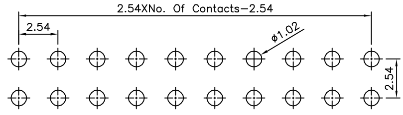
Recommended P.C.B. Layout(Top Side) (PCB Board Tolerance \pm 0.05 )
