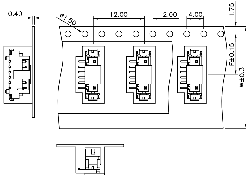
△ Carrier For 2~9Pin
