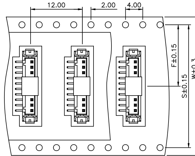
△ Carrier For 10~15Pin
