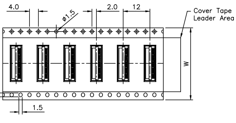
For Reel Width(Dimension W)32,44,56mm Double Row Hole
