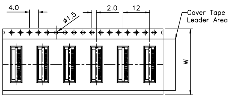
For Reel Width(Dimension W)16,24mm,Single Row Hole
