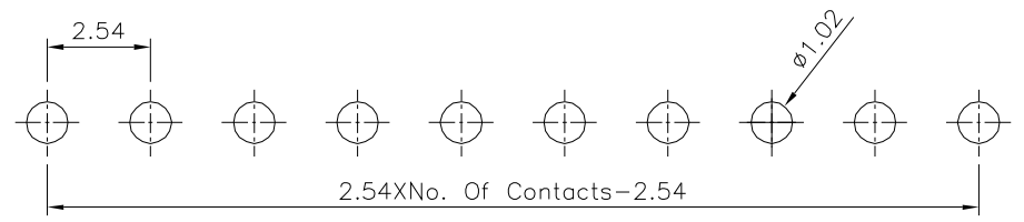
Recommended P.C.B. Layout(Top View) (PCB Board Tolerance±0.05)
