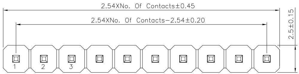
Recommended P.C.B. Layout(Top View) (PCB Board Tolerance±0.05)
