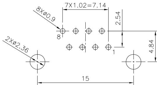
△ Recommended P.C.B. Layout (PCB Board Tolerance±0.05)
