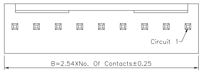
Recommended P.C.B. Layout Thickness 0.80~1.60mm
