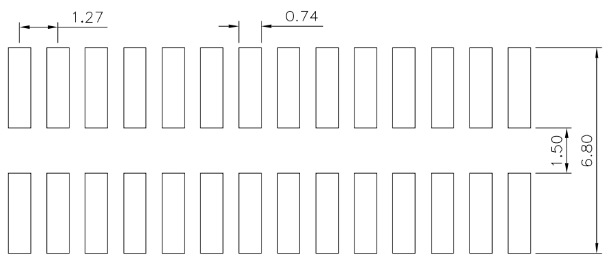
Recommended P.C.B. Layout (PCB Board Tolerance±0.05)
