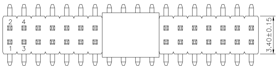
Recommended P.C.B. Layout (PCB Board Tolerance±0.05)
