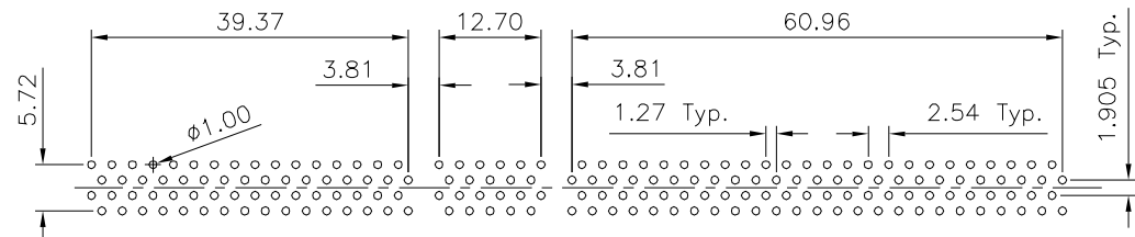
Recommended PCB Layout (Top View)
