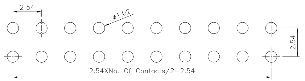
Recommended P.C.B. Layout(Top View) (PCB Board Tolerance±0.05)
