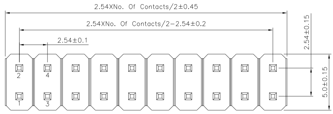
Recommended P.C.B. Layout(Top View) (PCB Board Tolerance±0.05)
