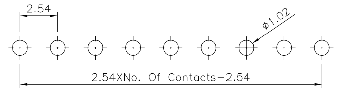
Recommended P.C.B. Layout Tolerance:±0.05(Top View)
