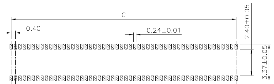
Recommended P.C.B. Layout (PCB Board Tolerance±0.03)
