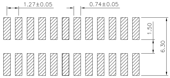
Recommended P.C.B Layout (PCB Board Tolerance±0.05)
