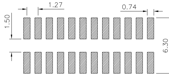
Recommended P.C.B. Layout (PCB Board Tolerance±0.05)
