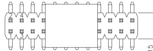
Recommended P.C.B. Layout (PCB Board Tolerance±0.05)
