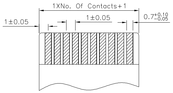
Proper Cable (Thickness: 0.3 \pm 0.02 mm)
