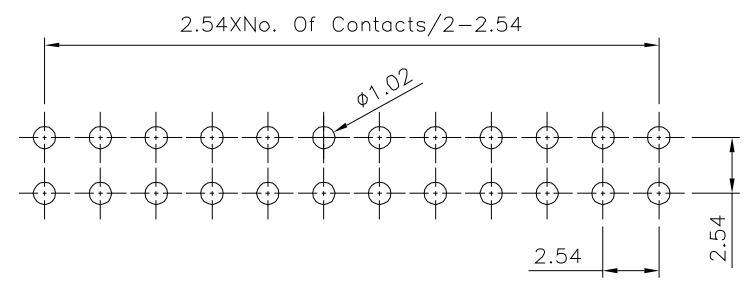
Recommended P.C.B. Layout PCB Tolerance: \pm 0.05 (Top View)
